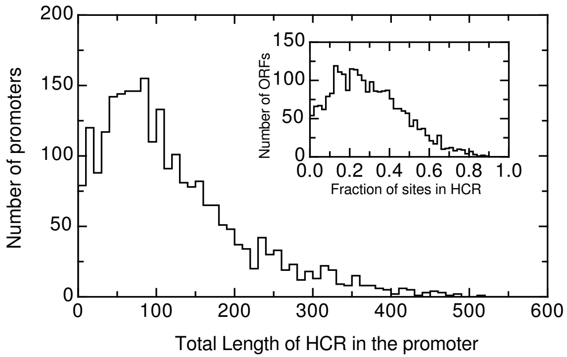
FIG. 1: Distribution of the total length of the high conservation regions over all promoters. For each promoter, we also calculated what fraction was in HCRs. The distribution of this HCR fraction is shown in the inset.
